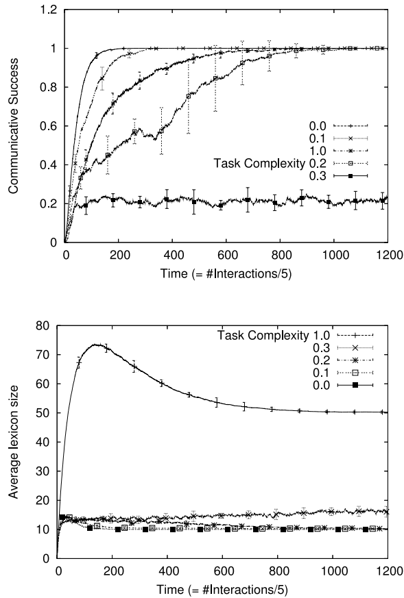
Figure 1. Influence of the task complexity on the evolution of the communicative success and the average lexicon size for several values of the task complexity. The curves were obtained for 5 agents, N_e = 5 and N_p = 5 , averaged over 10 independent runs.
